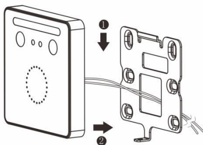
Figure1-5 KF1000 Series Installation
