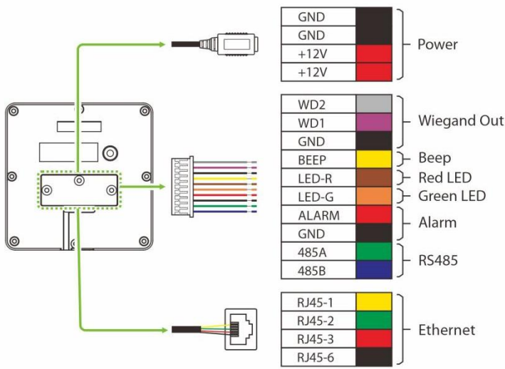
Figure 1-2 Terminal Description
